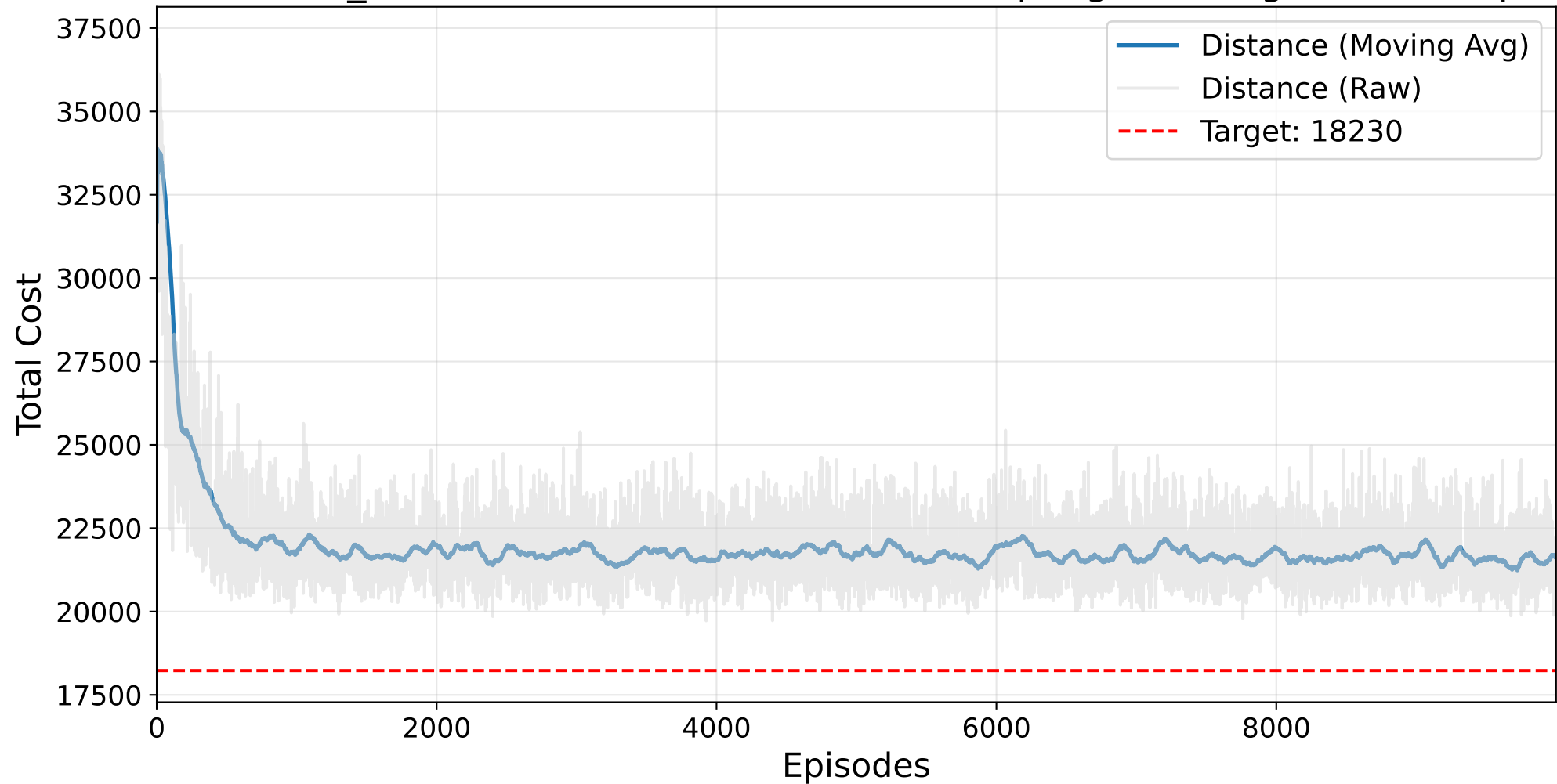
Final NO_MASK Masked AutoRL-SOP (Resampling) Training - ESC78.sop
